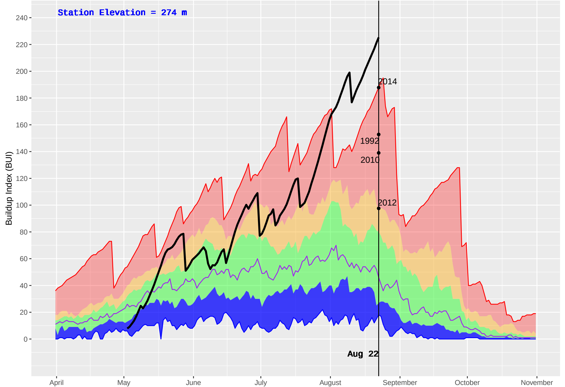
CEDARVALE (429) : Historical (1982–2016) and Current (2018) Daily Buildup Index (BUI)
